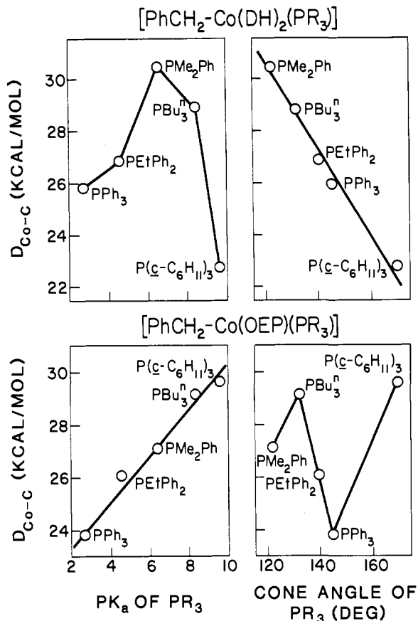
Figure 1. Dependence of D_{Co-C} on the pK_a and cone angle of PR_3 .
